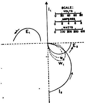
FIG. 5.—Constant Current, Step Down, Arm at 0^\circ
